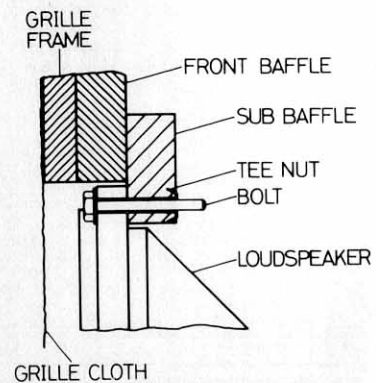
Loudspeaker Mounting Scale 1:8
